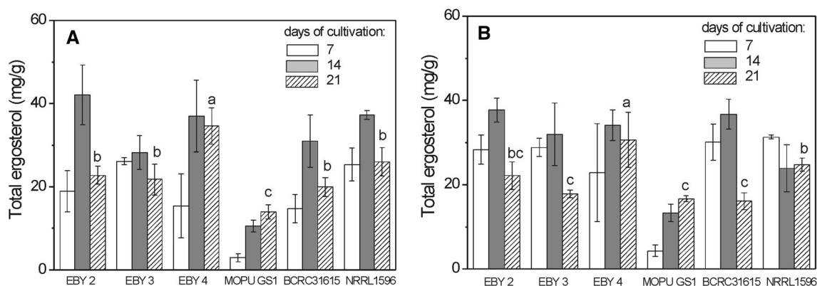
Fig. 2 Influence of rice (A) and millet (B) substrates on production of ergosterol by selected Monascus purpureus strains after 7, 14 and 21 days of fermentation. Data are mean \pm standard deviation ( n = 3 ). The amount of ergosterol was estimated based on the dry mass of the
