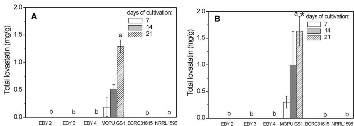
Fig. 3 Influence of rice (A) and millet (B) substrates on production of lovastatin by the selected Monascus purpureus strains after 7, 14 and 21 days of fermentation. Data are mean \pm standard deviation ( n = 3 ). The amount of lovastatin was estimated based on the dry
