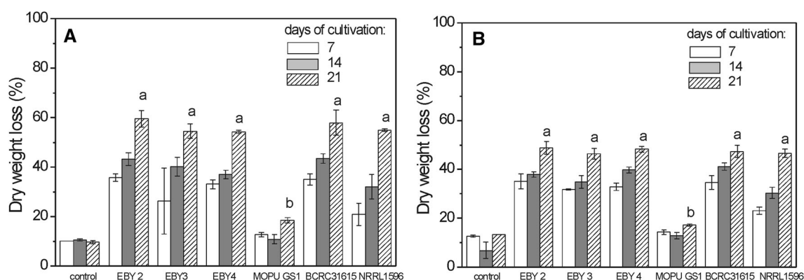
Fig. 1 Loss of dry matter of rice (A) and millet (B) substrates after 7, 14 and 21 days of fermentation with selected Monascus purpureus strains. Data are mean \pm standard deviation ( n = 3 ). Mean values
